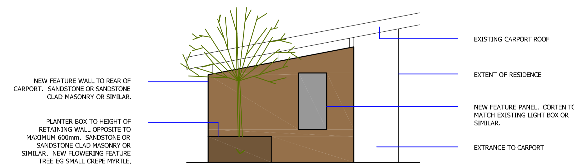
ELEVATION - ENTRANCE SCALE 1:50
